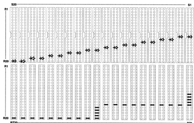
REMOTE-1 CARD #2
